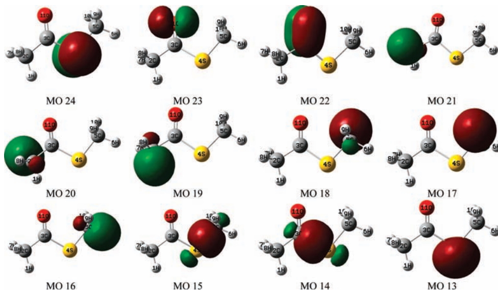
Figure 2. Characters of the 12 highest occupied molecular orbitals of CH 3 C(O)SCH 3 . The trend following Table 1 is from MO 24 [ n '(S)] to MO 13 [ n ' o (S)].
